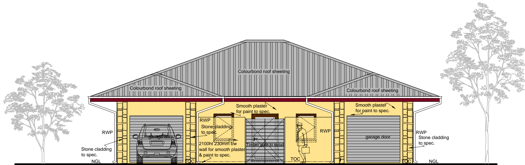
ELEVATION 1-1
